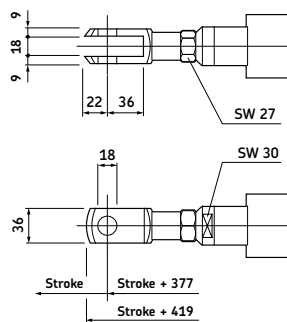
Fork head
