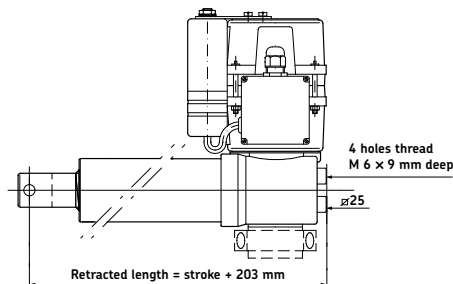
Rear screw fixing
