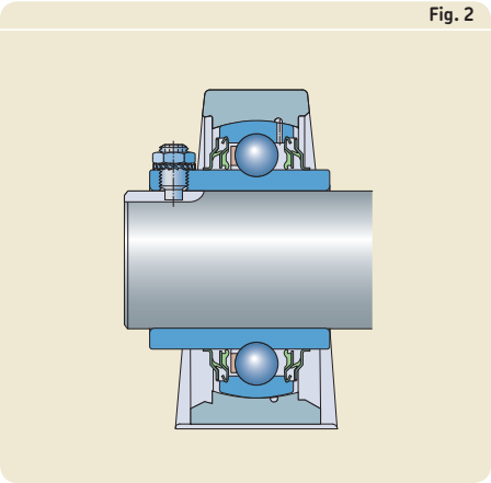
Threaded holes in the inner ring of YAR and YAT bearings
