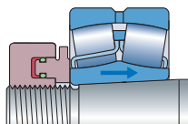
One sliding surface
