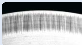
Fluting marks characteristic of electrical erosion in bearings
