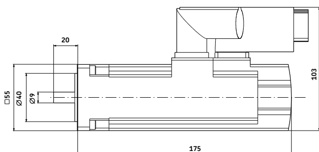
Dimensional drawing Siemens motor 1FK7022
