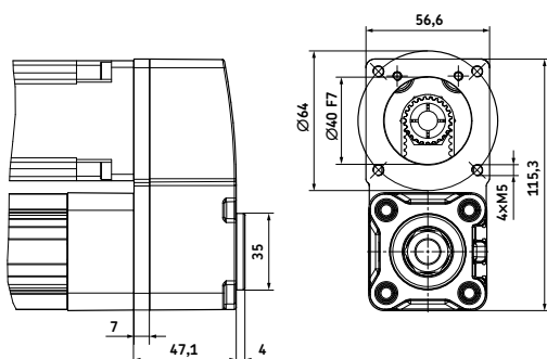
Parallel adapter kit for CASM-40 and Siemens 1FK7022 motor*
