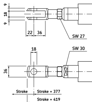
Front attachment
