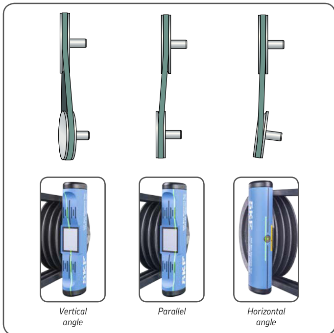
Figure 5 Misalignment summary
